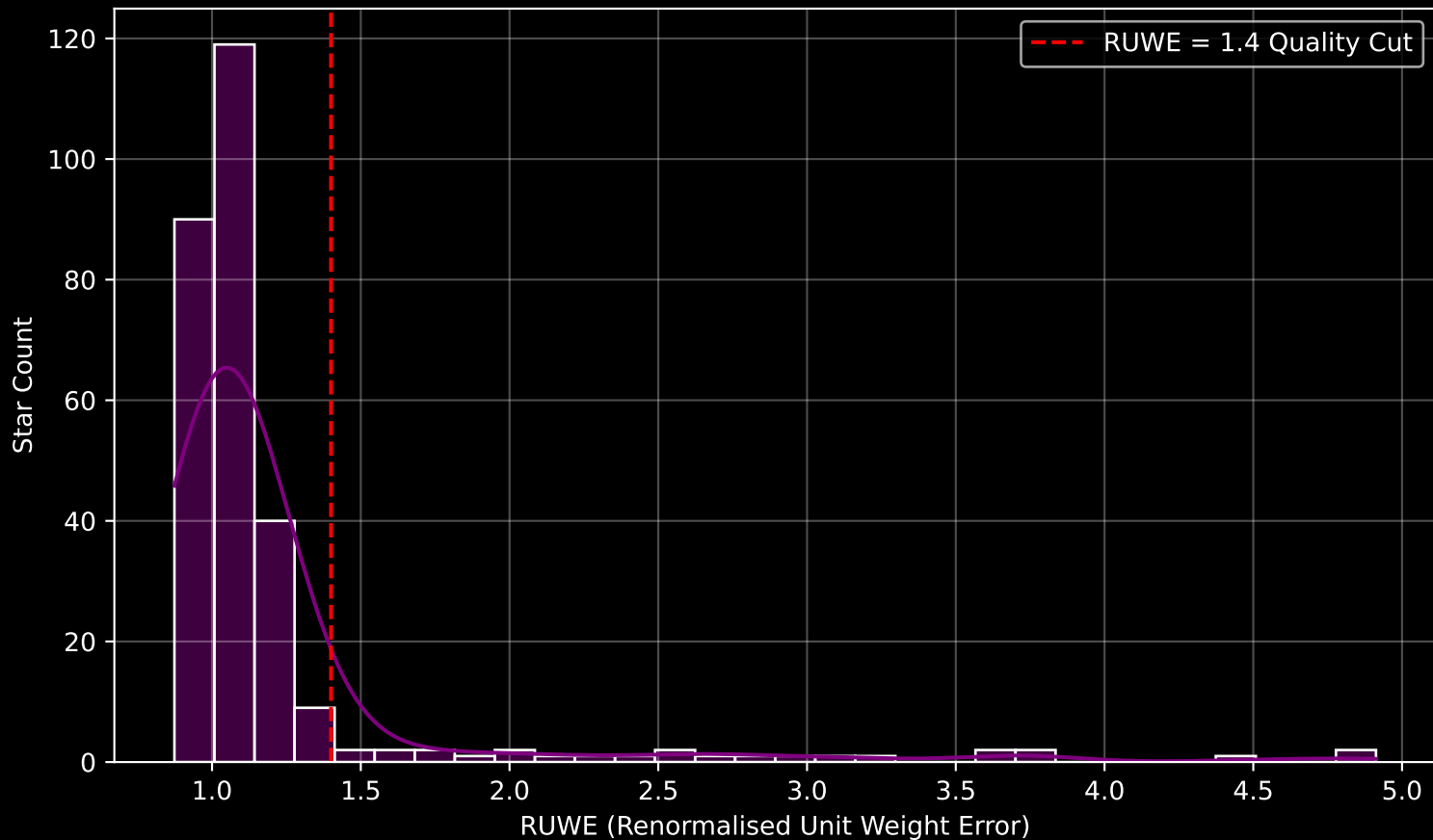
GALAH DR4 Field [1079] RUWE Distribution (n= 284)
