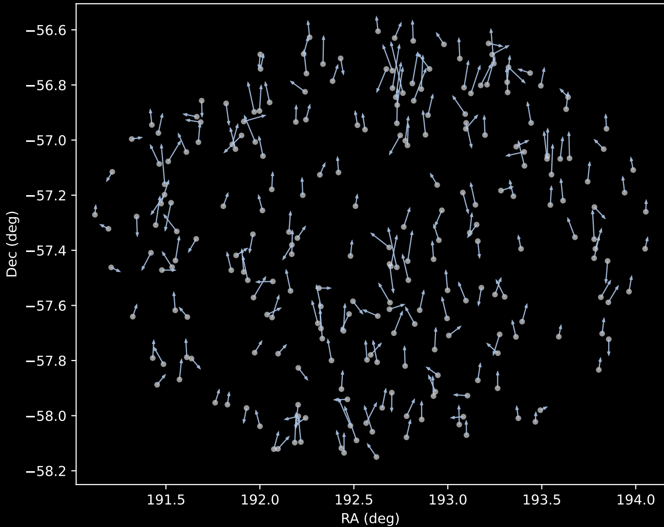
GALAH DR4 Cluster 1 Proper Motion Vectors (n=240)
