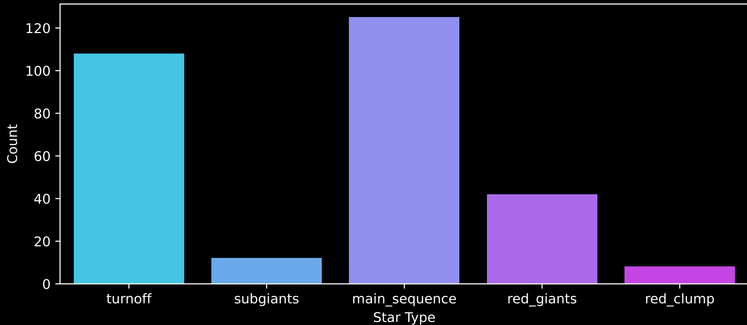
GALAH DR4 Field: [1079] Count plot of Star Type
